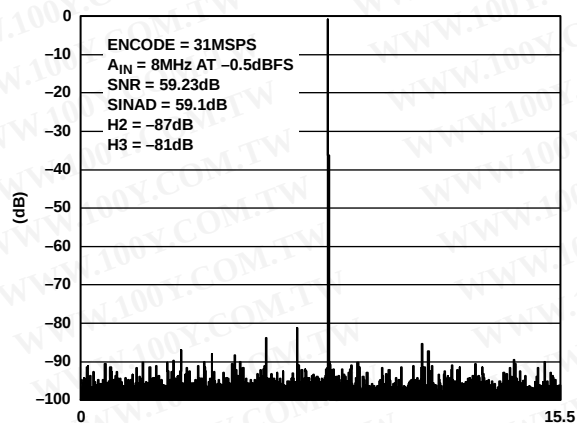
Figure 20. FFT: F_S = 31 MSPS, A_{IN} = 8 MHz @ -0.5 dBFS, Differential, 1 V p-p Input Range
