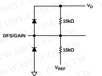
Figure 13. DFS/Gain Input
