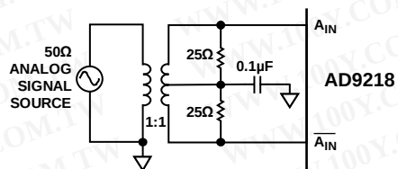
Figure 42. Using a Wideband Transformer to Drive the AD9218
