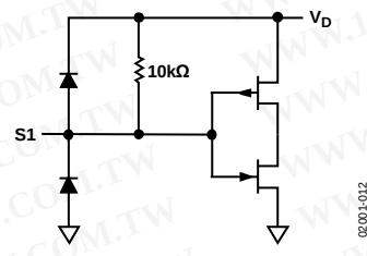
Figure 12. S1 Input
