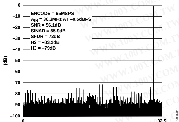
Figure 16. FFT: FS = 65 MSPS, A_{IN} = 30.3\text{ MHz @ } -0.5\text{ dBFS} , Differential, 2 V p-p Input Range
