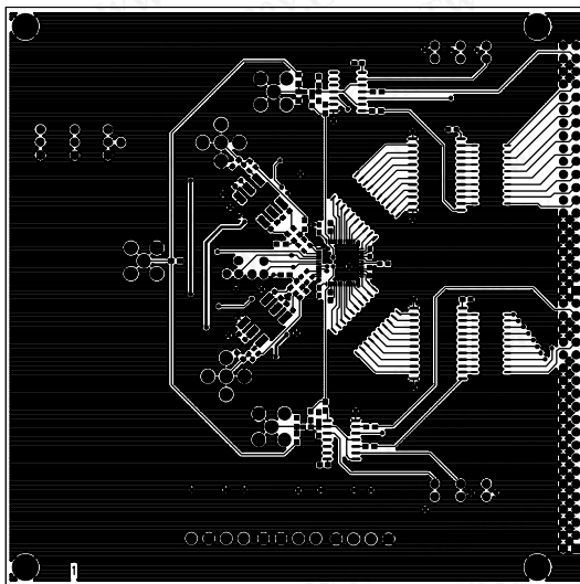
Figure 48. Top Routing
