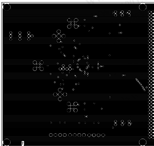
Figure 49. Ground Plane
