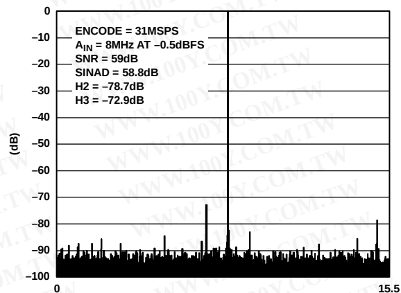
Figure 23. FFT: F_S = 31 MSPS, A_{IN} = 8 MHz @ -0.5 dBFS, Differential, with AD8138 Driving ADC Inputs, 1 V p-p Input Range
