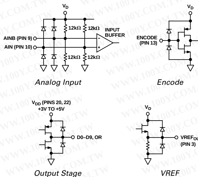
Figure 2. Equivalent Circuits
