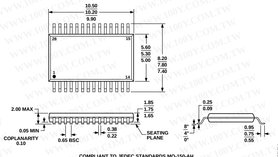
Figure 7.28—Lead Shrink Small Outline Package [SSOP] (RS-28)
