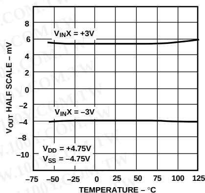
Figure 6. V_{OUT} Half Scale ( 80_H ) vs. Temperature
