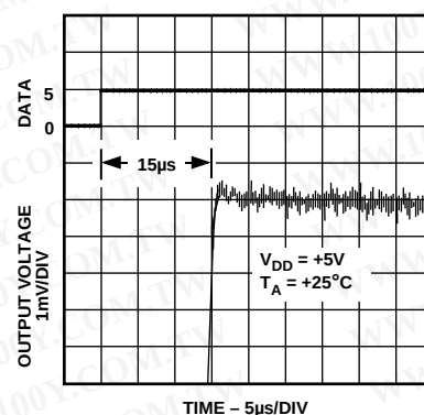
Figure 13. Output Voltage Rise Time Detail
