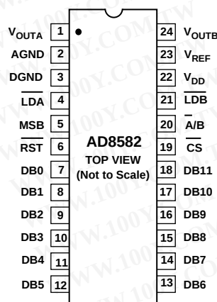
N-24 24-Pin Plastic DIP
