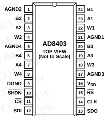
Figure 8. AD8403 Pin Configuration
