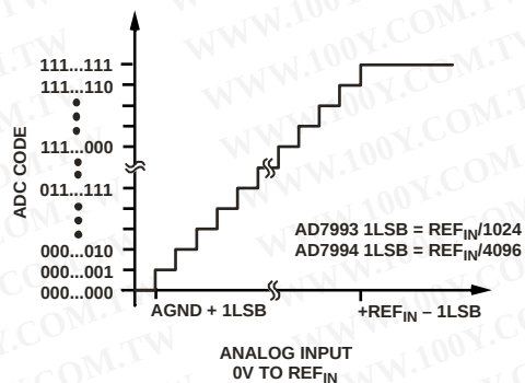
Figure 20. AD7993/AD7994 Transfer Characteristic
