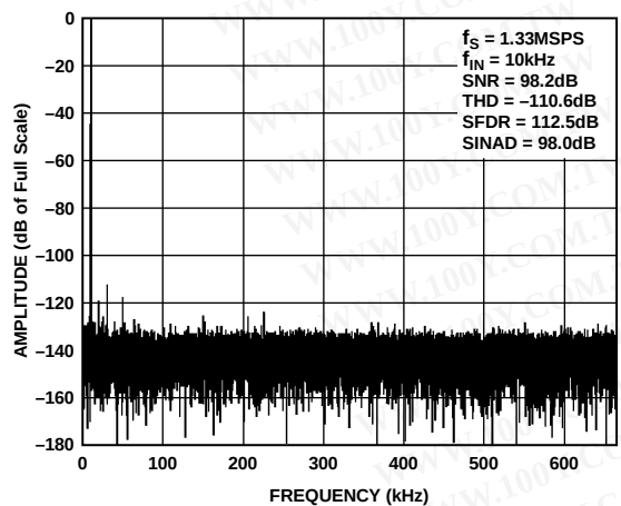
Figure 8. FFT Plot
