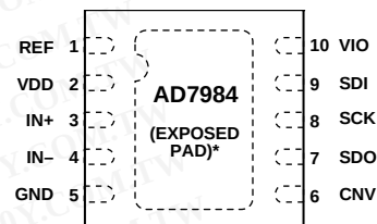
Figure 5. 10-Lead QFN (LFCSP) Pin Configuration
