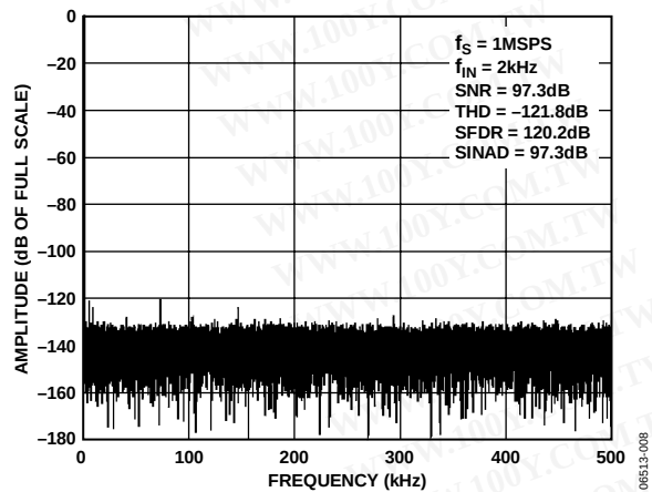
Figure 8. FFT Plot
