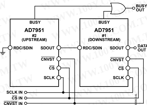
Figure 41. Two AD7951 Devices in a Daisy-Chain Configuration
