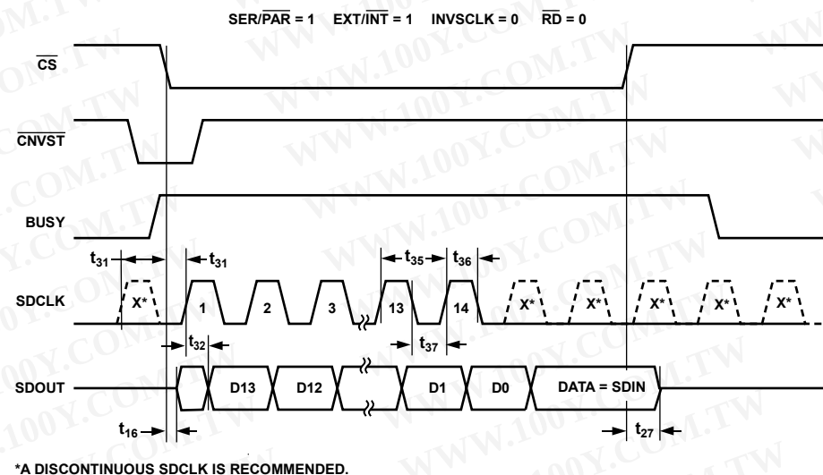
Figure 43. Slave Serial Data Timing for Reading (Read Previous Conversion During Convert)
