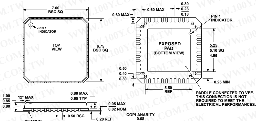
COMPLIANT TO JEDEC STANDARDS MO-220-VKDD-2 Figure 48. 48-Lead Lead Frame Chip Scale Package [LFCSP_VQ] 7 mm × 7 mm Body, Very Thin Quad (CP-48-1) Dimensions shown in millimeters
