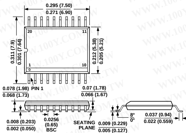
20-Lead SSOP (RS-20)
