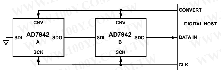
Figure 38. Chain Mode Without Busy Indicator Connection Diagram
