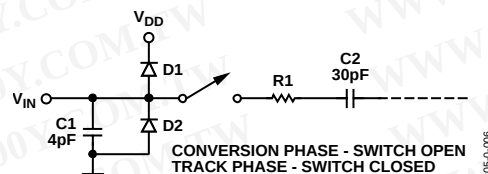
Figure 13. Equivalent Analog Input Circuit
