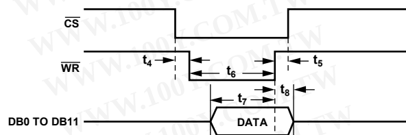
Figure 36. AD7933/AD7934 Parallel Interface—Write Cycle Timing for Word Mode Operation ( \overline{W/B} = 1 )
