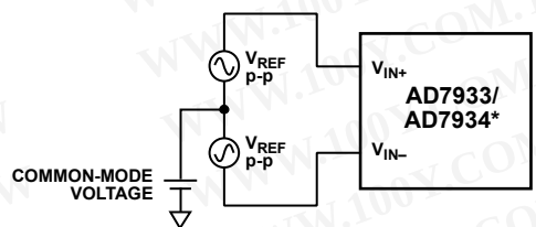
*ADDITIONAL PINS OMITTED FOR CLARITY. Figure 24. Differential Input Definition
