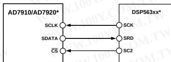
Figure 27. Interfacing to the DSP563xx
