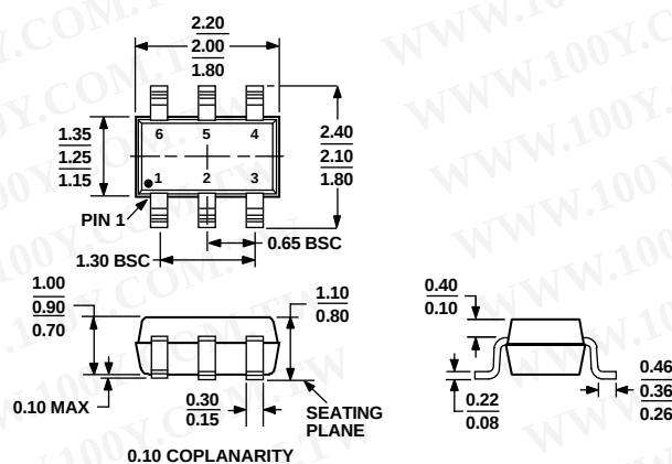
Figure 30. 6-Lead Thin Shrink Small Outline Transistor Package [SC70] (KS-6)
