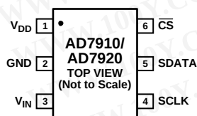
Figure 5. 6-Lead SC70 Pin Configuration
