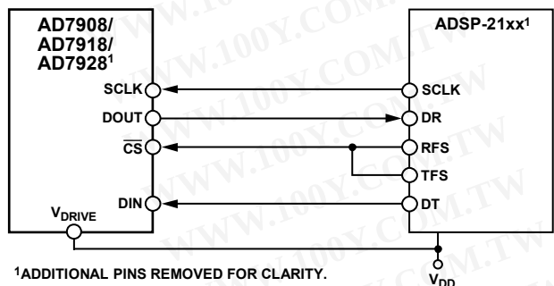
Figure 31. Interfacing to the ADSP-21xx
