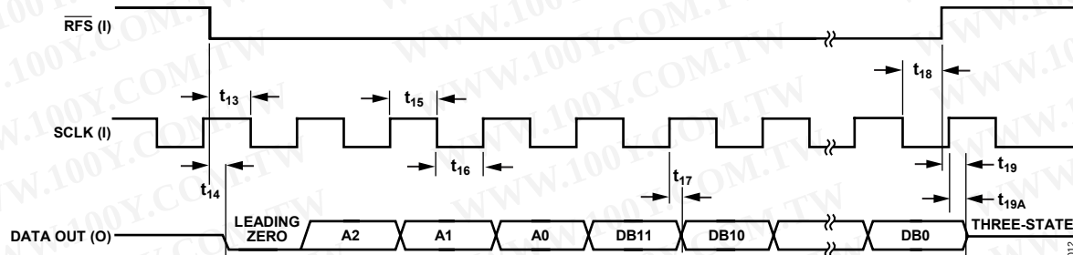
Figure 12. External Clocking (Slave) Mode Output Register Read
