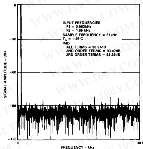
Figure 14. IMD Plot
