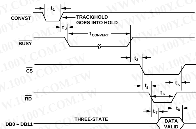
Figure 1. Timing Diagram
