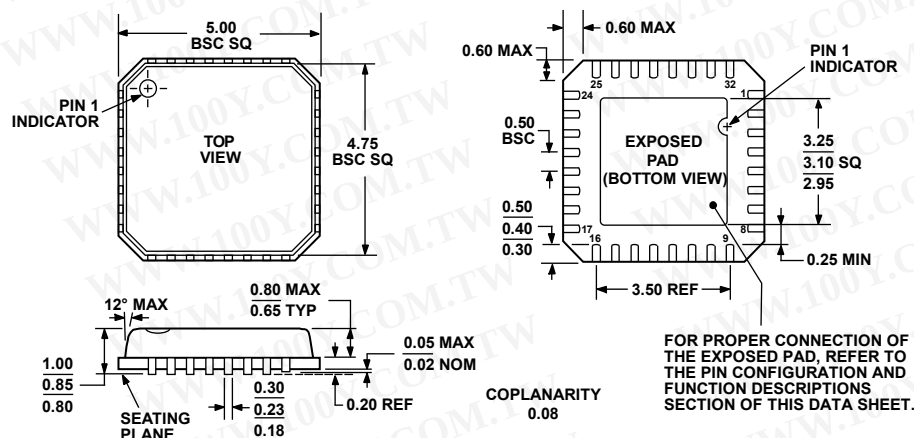
COMPLIANT TO JEDEC STANDARDS MO-220-VHDD-2 Figure 49. 32-Lead Lead Frame Chip Scale Package [LFCSP_VQ] 5 mm x 5 mm Body, Very Thin Quad (CP-32-2) Dimensions shown in millimeters
