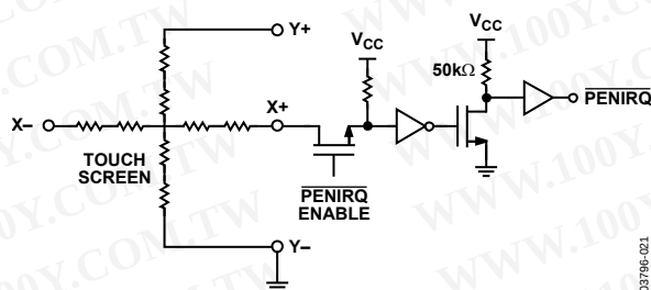
Figure 43. PENIRQ Output Equivalent Circuit
