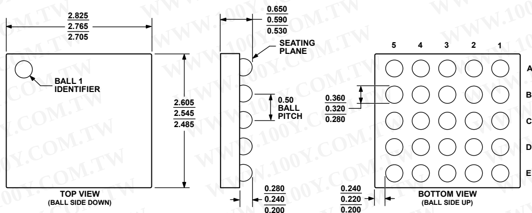
Figure 50. 25-Ball Wafer Level Chip Scale Package [WLCSPP] 2.5 mm x 2.8 mm Body (CB-25-1) Dimensions shown in millimeters
