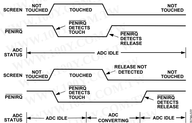
Figure 44. PENIRQ Operation for ADC Idle and ADC Converting
