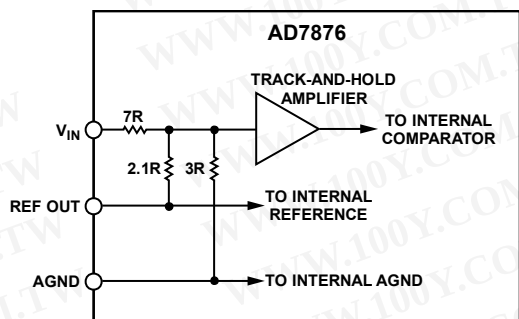
Figure 9. AD7876 Analog Input
