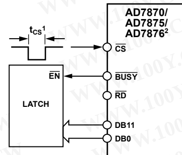
Figure 30. Stand-Alone Operation
