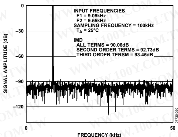
Figure 20. IMD Plot
