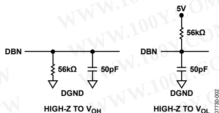
Figure 4. Load Circuits for Access Time
