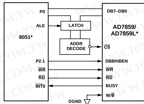
Figure 42. AD7859/AD7859L to 8051 Parallel Interface
