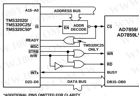
Figure 39. AD7859/AD7859L to TMS32020/C25/C5x Parallel Interface
