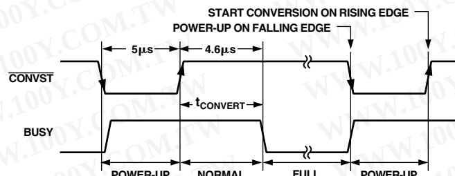
Figure 21. Using the \overline{CONVST} Pin to Power Up the AD7854 for a Conversion
