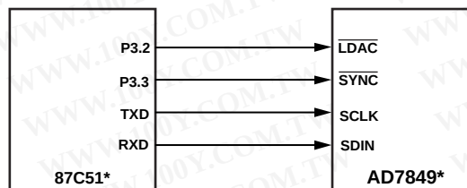
Figure 27. AD7849-to-87C51 Interface
