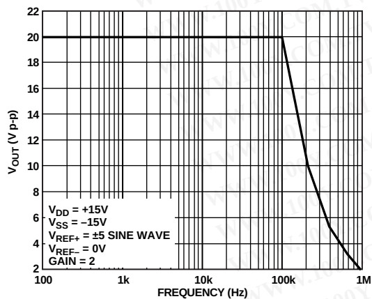
Figure 5. Large Signal Frequency Response
