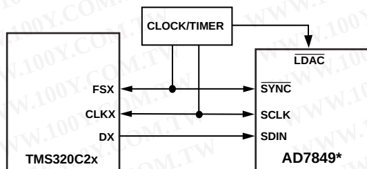
Figure 25. AD7849-to-TMS320C2x Interface
