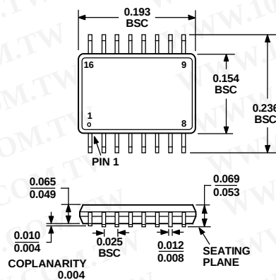
Figure 30. 16-Lead Shrink Small Outline Package [QSOP] (RQ-16)
