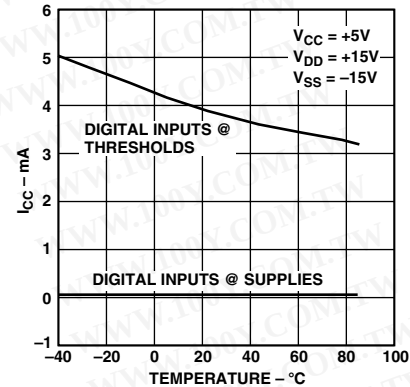
TPC 6. I_{CC} vs. Temperature
