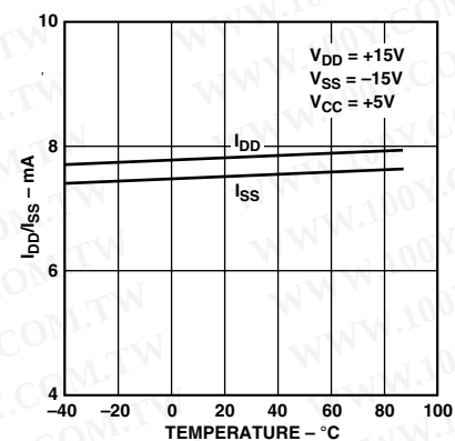
TPC 9. I_{DD} , I_{SS} vs. Temperature
