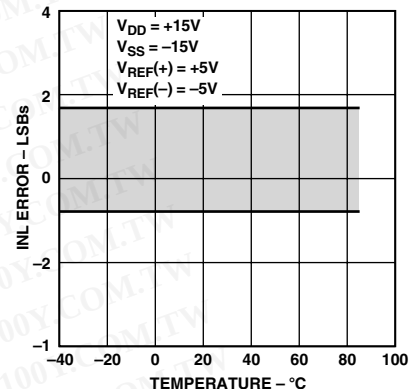
TPC 3. Typical INL Error vs. Temperature
