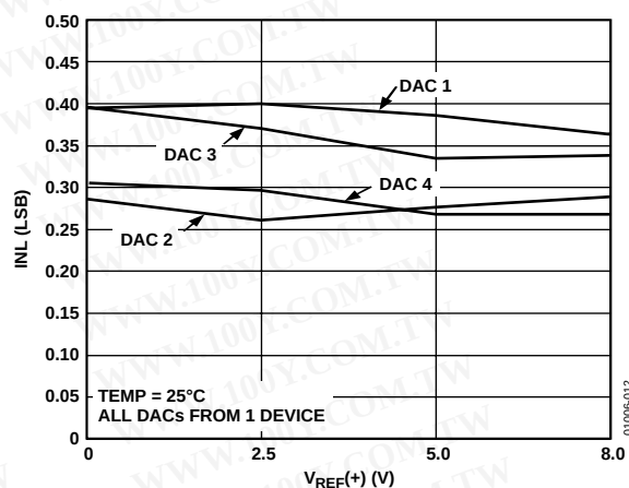
Figure 12. Typical INL vs. V_{REF}(+) , V_{REF}(+) - V_{REF}(-) = 5V
