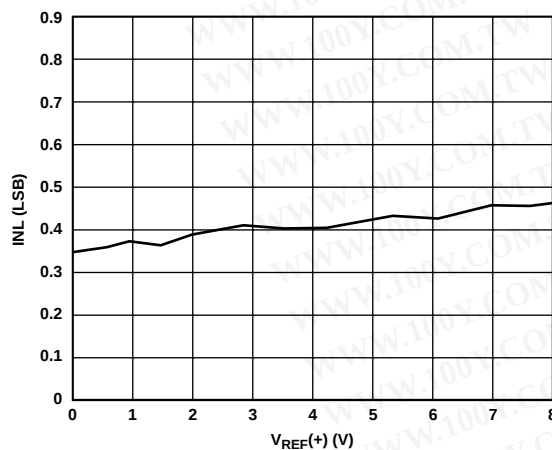
Figure 11. Typical INL vs. V_{REF}(+) , V_{REF}(-) = -6V
