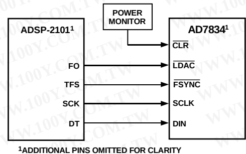
Figure 28. AD7834 to ADSP-2101 Interface
