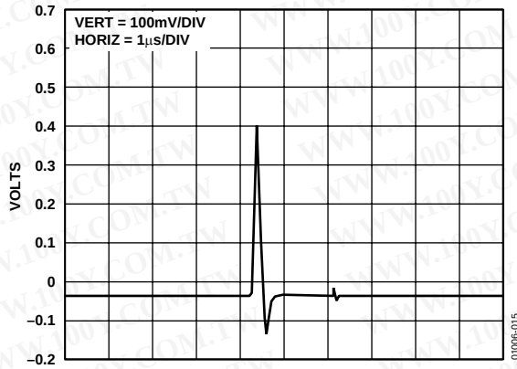
Figure 15. Typical Digital/Analog Glitch Impulse
