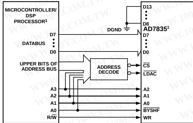
Figure 32. AD7835 8-Bit Interface
