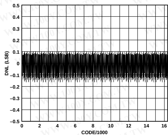
Figure 10. Typical DNL Plot
