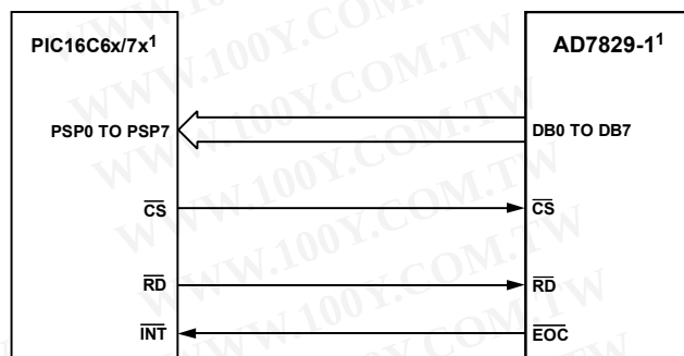
Figure 25. Interfacing to the PIC16C6x/PIC16C7x
