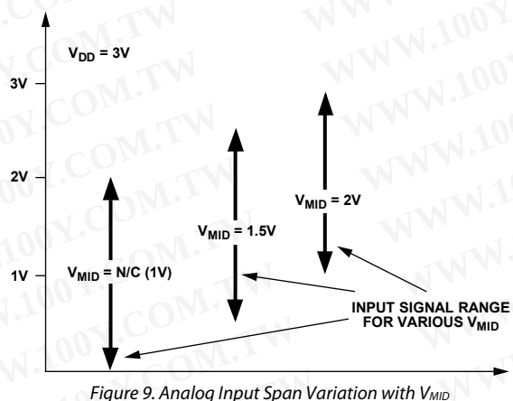
Figure 9. Analog Input Span Variation with V_{MID}
