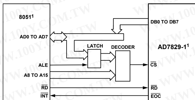
Figure 24. Interfacing to the 8051
