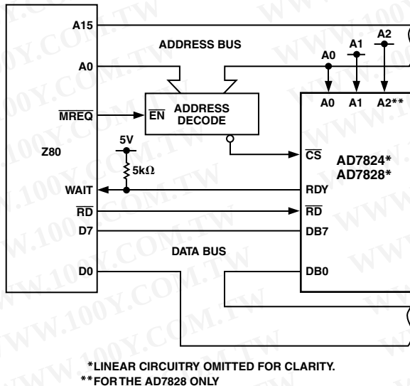
Figure 16. AD7824/AD7828–Z80 Interface
