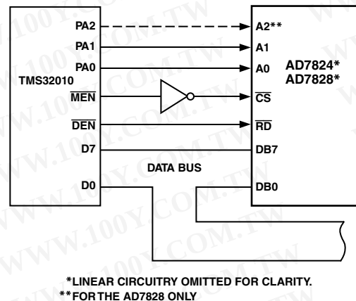
Figure 18. AD7824/AD7828–TMS32010 Interface
