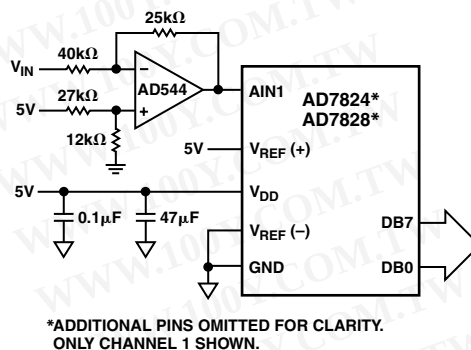
Figure 12. AD7824/AD7828 Bipolar \pm 4 V Operation
