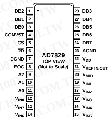
Figure 5. Pin Configuration
