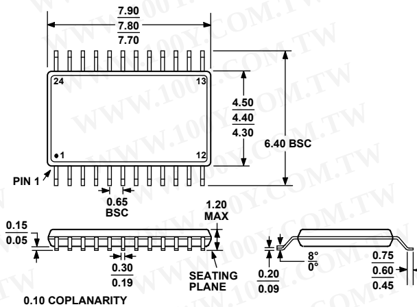
Figure 37. 24-Lead Thin Shrink Small Outline Package [TSSOP]
