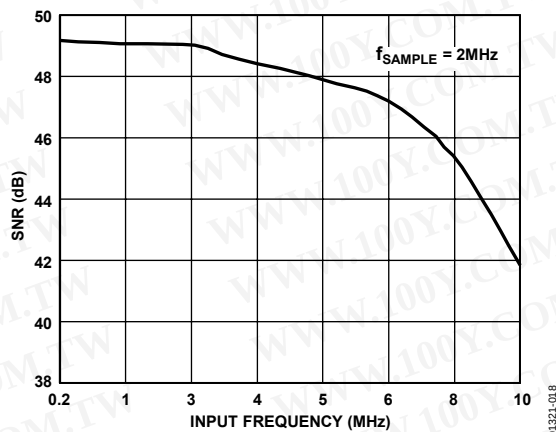
Figure 18. SNR vs. Input Frequency on the AD7829
