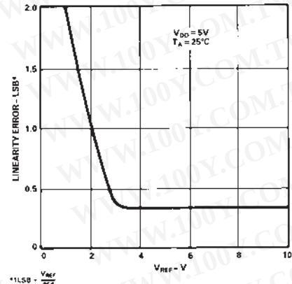
TPC 6. Accuracy vs. V_{REF} [ V_{REF} = V_{REF(+)} - V_{REF(-)} ]
