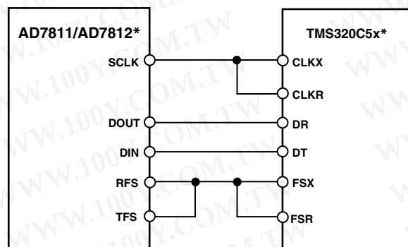
Figure 23. Interfacing to the TMS320C5x
