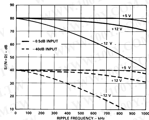
Figure 18. Power Supply Rejection ( f_{IN} = 10 kHz, f_{SAMPLE} = 128 kSPS, V_{RIPPLE} = 0.1 V p-p)
