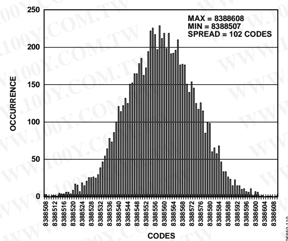
Figure 24. AD7767-1 24-Bit Histogram
