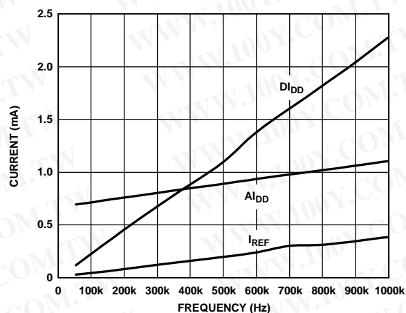
Figure 44. AD7767-1 Current vs. MCLK Frequency
