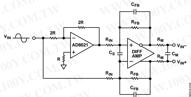
Figure 37. Single-Ended-to-Differential Conversion
