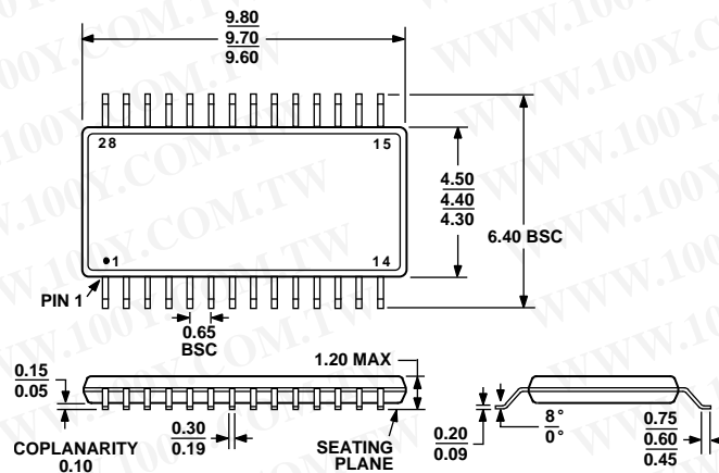
COMPLIANT TO JEDEC STANDARDS MO-153-AE Figure 54. 28-Lead Thin Shrink Small Outline [TSSOP] (RU-28) Dimensions shown in millimeters
