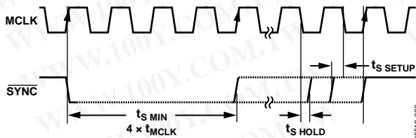
Figure 41. SYNC Timing Relative to MCLK
