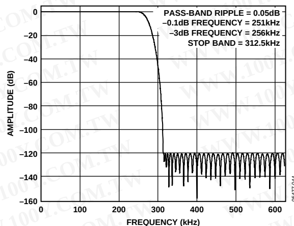
Figure 31. Default Filter Frequency Response (625 kHz ODR)
