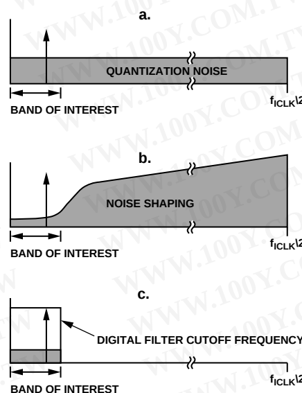
Figure 22. \Sigma - \Delta ADC
