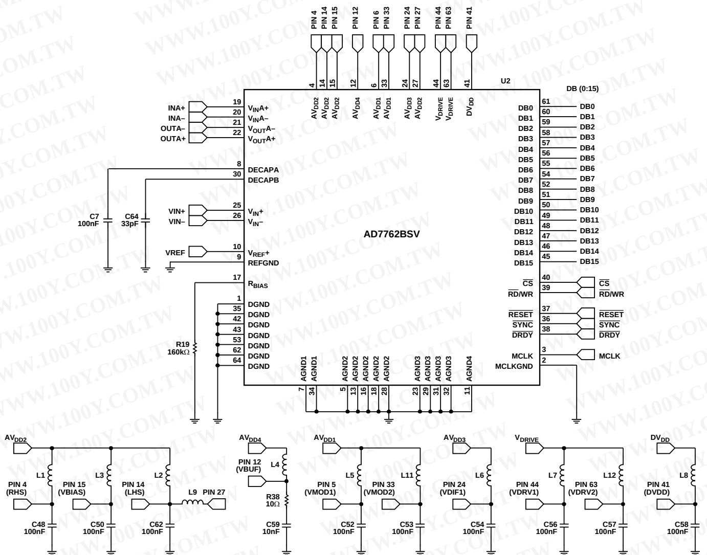
Figure 29. Simplified Connection Diagram
