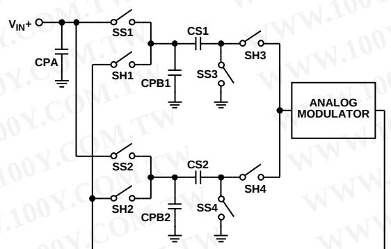
Figure 28. Equivalent Input Circuit
