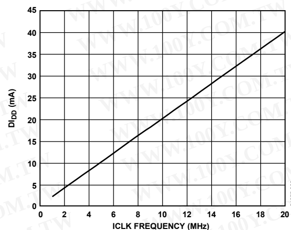
Figure 39. Decimate \times 256 , DI_{DD} vs. ICLK Frequency ( DV_{DD} = 2.5\text{ V} )
