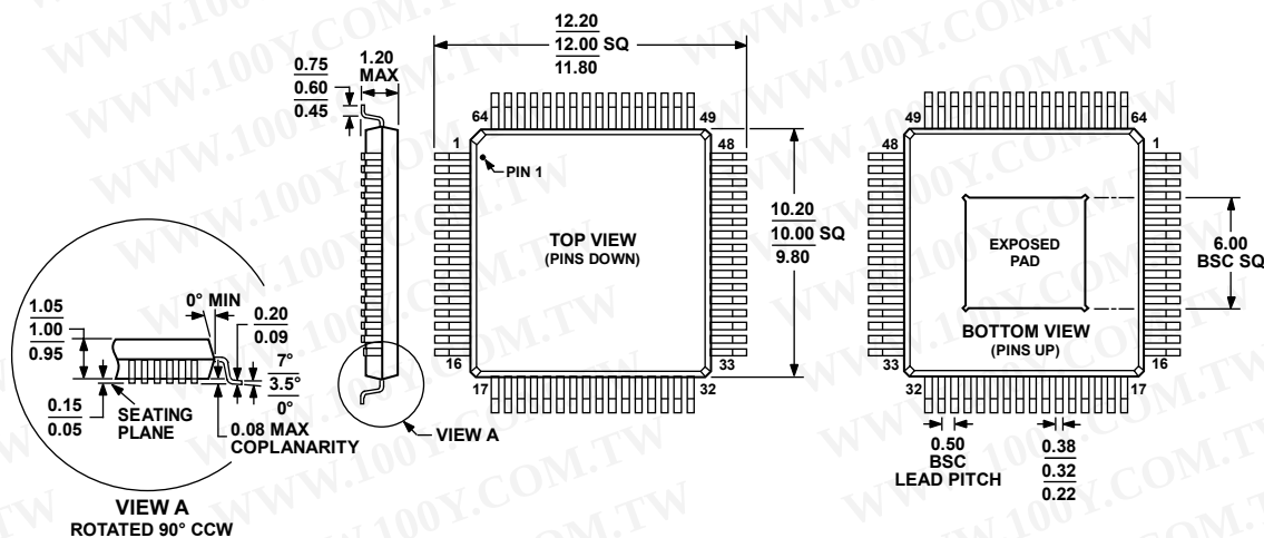
Figure 59. 64-Lead Thin Quad Flat Package, Exposed Pad [TQFP_EP] (SV-64-2)
