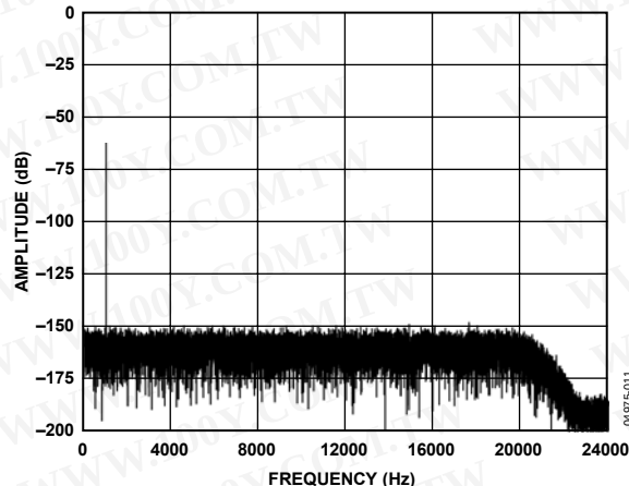
Figure 10. Low Power FFT, 1 kHz, -60 dB Input Tone, 256x Decimation
