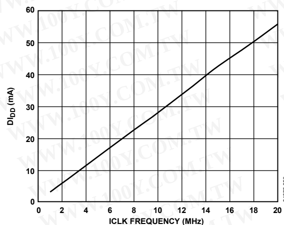
Figure 37. Decimate \times 8 , DI_{DD} vs. ICLK Frequency ( DV_{DD} = 2.5\text{ V} )
