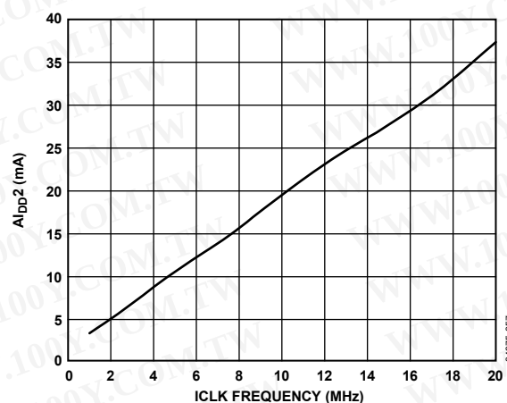
Figure 36. AI_{DD2} vs. ICLK Frequency ( AV_{DD2} = 5\text{ V} )
