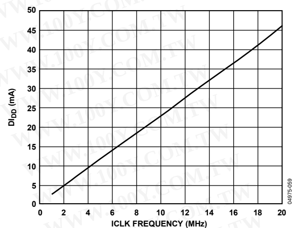
Figure 38. Decimate \times 32 , DI_{DD} vs. ICLK Frequency ( DV_{DD} = 2.5\text{ V} )
