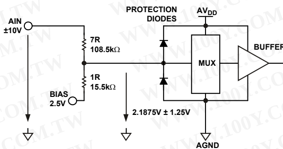
Figure 23. Simplified Analog Input Internal Structure
