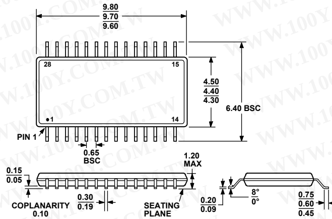
Figure 31. 28-Lead This Shrink Small Outline Package [TSSOP] (RU-28)—Dimensions shown in millimeters
