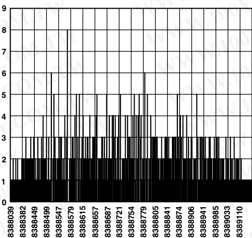
TPC 2. AD7718 Noise Distribution Histogram
