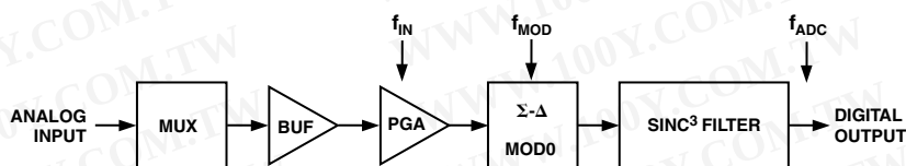
Figure 10. ADC Channel Block Diagram with CHOP Disabled
