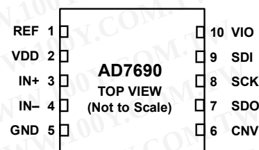
Figure 6. 10-Lead QFN (LFCSP) Pin Configuration
