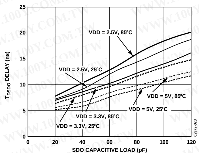
Figure 24. t_{SDO} Delay vs. Capacitance Load and Supply
