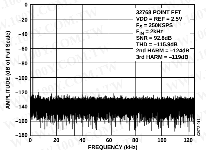
Figure 12. FFT Plot
