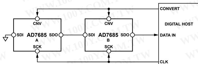
Figure 42. Chain Mode Connection Diagram
