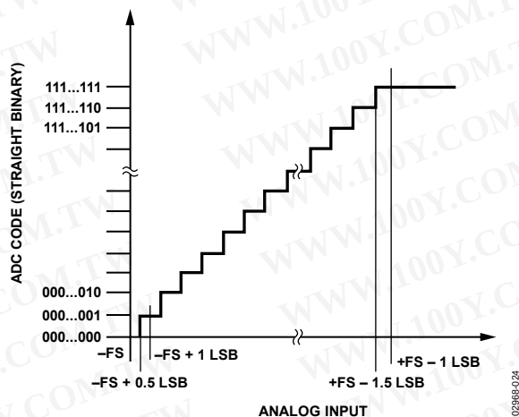
Figure 26. ADC Ideal Transfer Function
