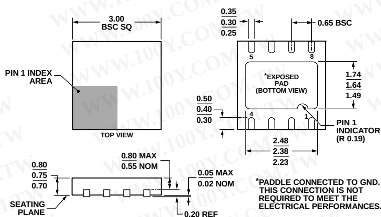
Figure 27. 8-Terminal Quad Flat No Lead Package (QFN) [LFCSP_WD] 3 mm × 3 mm Body, Very Very Thin, Dual Lead (CP-8-3)
