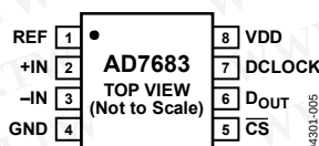
Figure 6. 8-Lead MSOP and QFN (LFCSP) Pin Configuration
