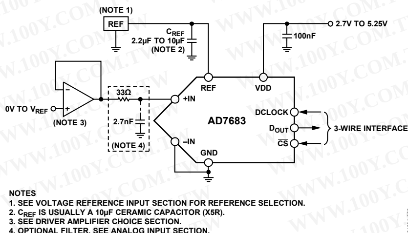
Figure 22. Typical Application Diagram
