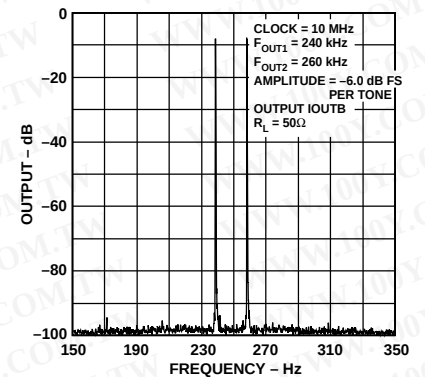
Figure 20. Intermodulation Distortion
