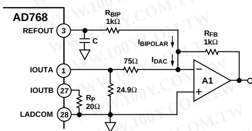
Figure 25. Bipolar \pm 2.5 V Buffered Voltage Output
