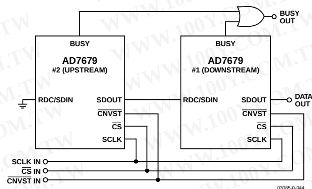
Figure 42. Two AD7679s in a Daisy-Chain Configuration
