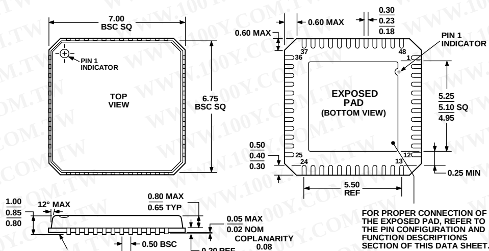
Figure 45. 48-Lead Lead Frame Chip Scale Package [LFCS_P_VQ] 7 mm × 7 mm Body, Very Thin Quad (CP-48-1) Dimensions shown in millimeters
