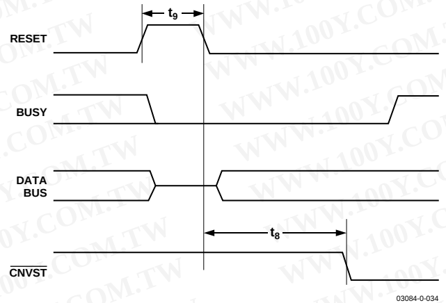
Figure 28. RESET Timing
