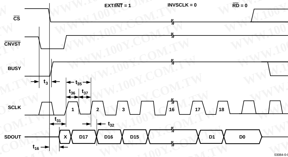
Figure 36. Slave Serial Data Timing for Reading (Read Previous Conversion during Convert)
