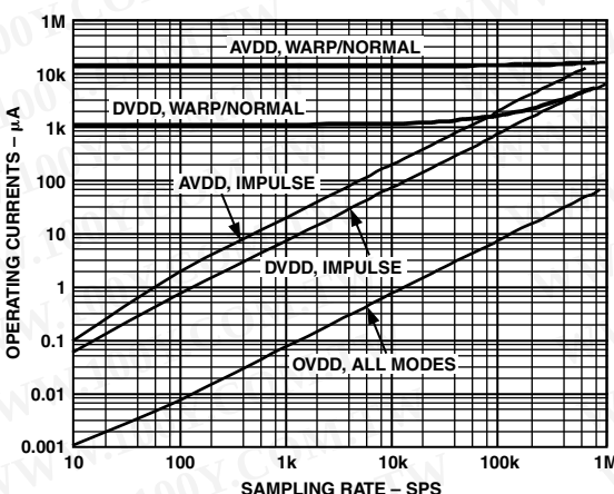
TPC 12. Operating Currents vs. Sample Rate
