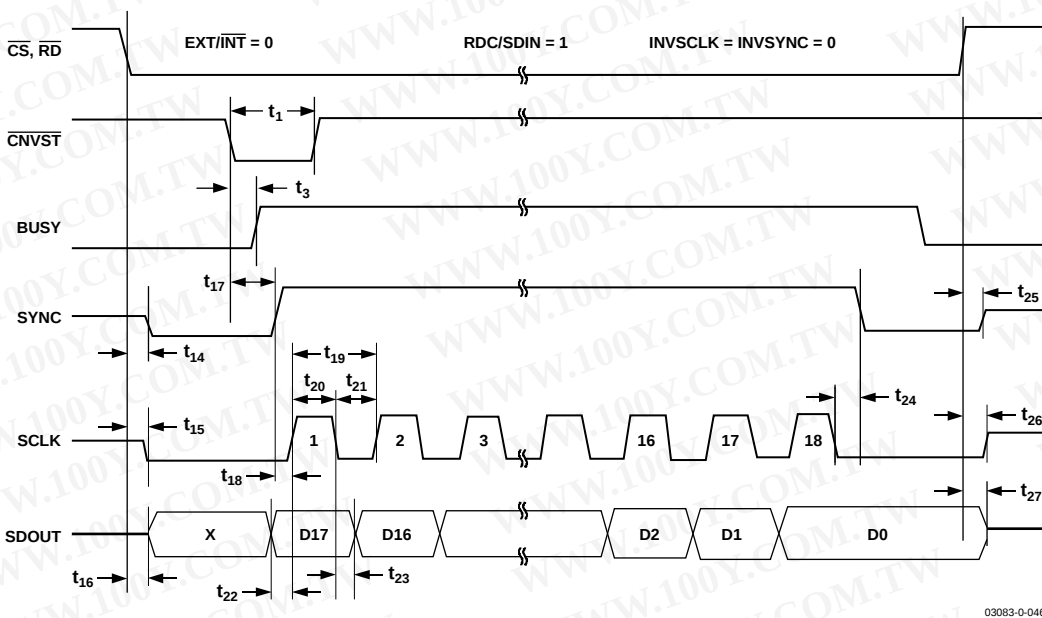
Figure 41. Master Serial Data Timing for Reading (Read Previous Conversion during Convert)
