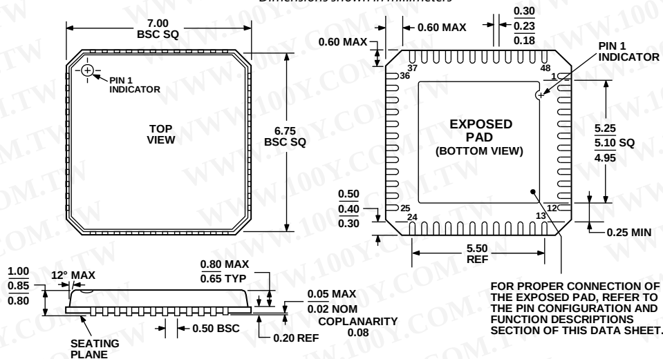
COMPLIANT TO JEDEC STANDARDS MO-220-VKGD-2 Figure 47. 48-Lead Lead Frame Chip Scale Package [LFCSP_VQ] 7 x 7 mm Body, Very Thin Quad (CP-48-1)
