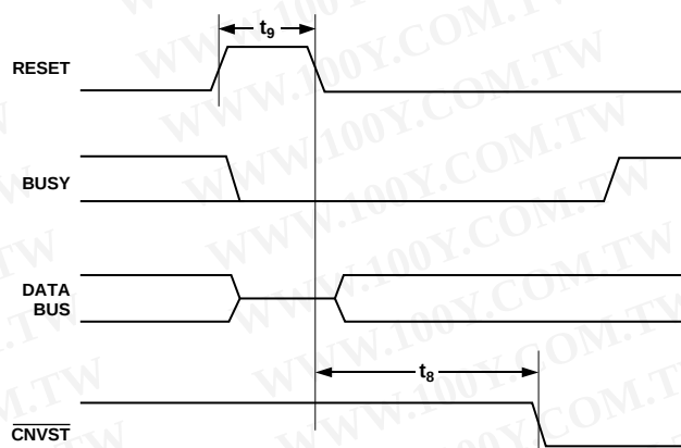
Figure 35. RESET Timing
