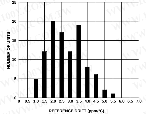
Figure 22. Reference Voltage Temperature Coefficient Distribution (102 Units)
