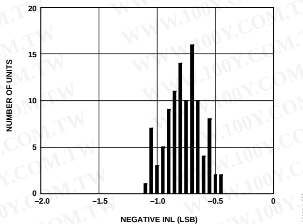
Figure 9. Typical Negative INL Distribution (102 Units)
