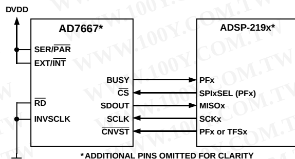
Figure 44. Interfacing the AD7667 to an SPI Interface
