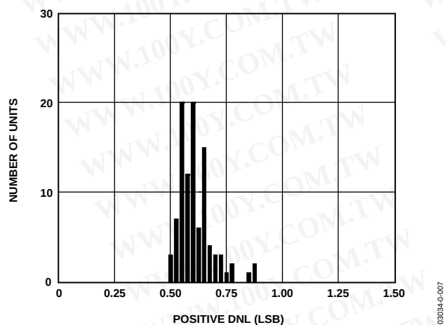
Figure 7. Typical Positive DNL Distribution (99 Units)
