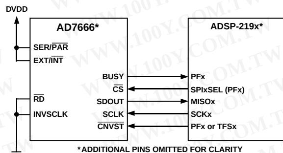
Figure 44. Interfacing the AD7666 to an SPI Interface
