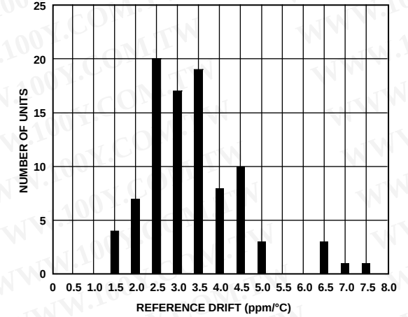
Figure 22. Reference Voltage Temperature Coefficient Distribution (93 Units)
