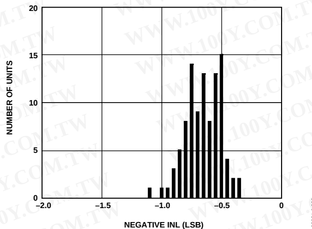
Figure 9. Typical Negative INL Distribution (99 Units)
