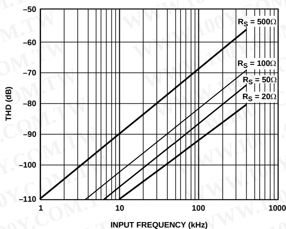
Figure 29. THD vs. Analog Input Frequency and Source Resistance
