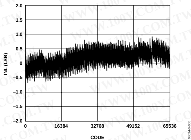
Figure 5. Integral Nonlinearity vs. Code
