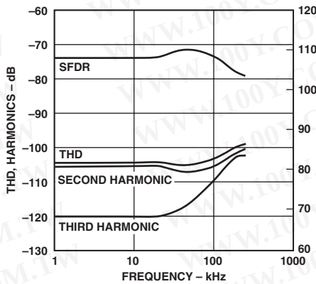
TPC 8. THD, Harmonics, and SFDR vs. Frequency
