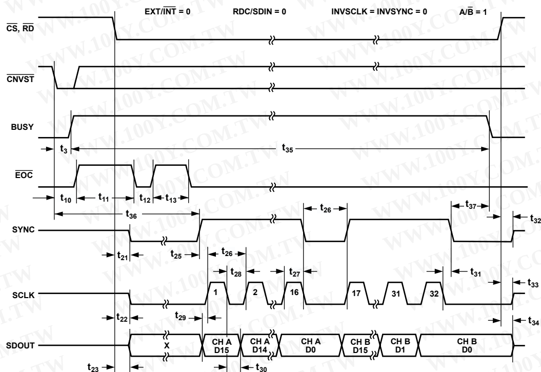
Figure 29. Master Serial Data Timing for Reading (Read After Conversion)
