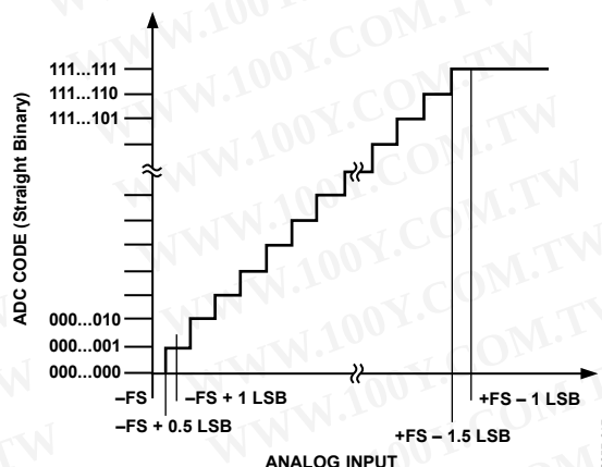
Figure 17. ADC Ideal Transfer Function
