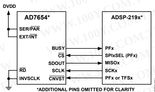
Figure 34. Interfacing the AD7654 to an SPI Interface
