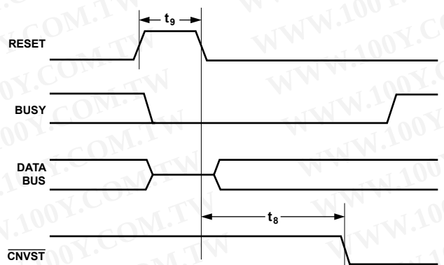
Figure 23. Reset Timing
